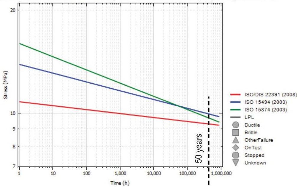
Comparison of PE-100, PP and PE-RT (type II) at 20°C
