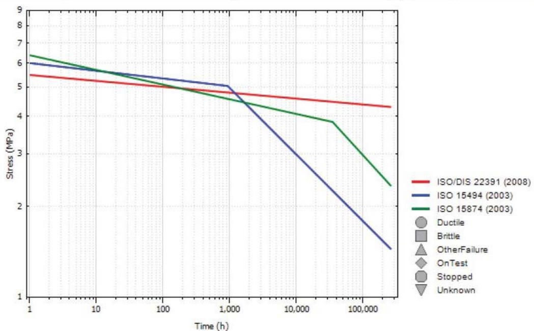
Comparison of PE-100, PP and PE-RT (type II) at 80°C
