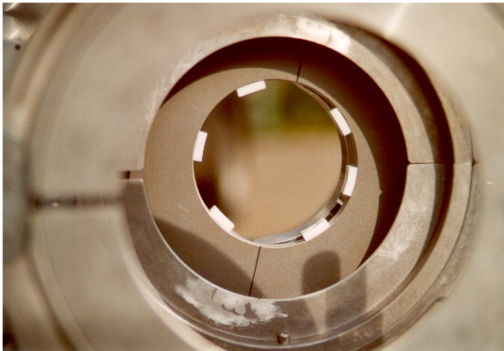
Devided welding mirror with distance spacer
