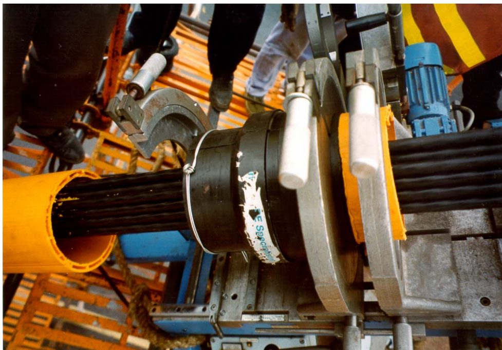
Pylon fixing unit for half-pipe
