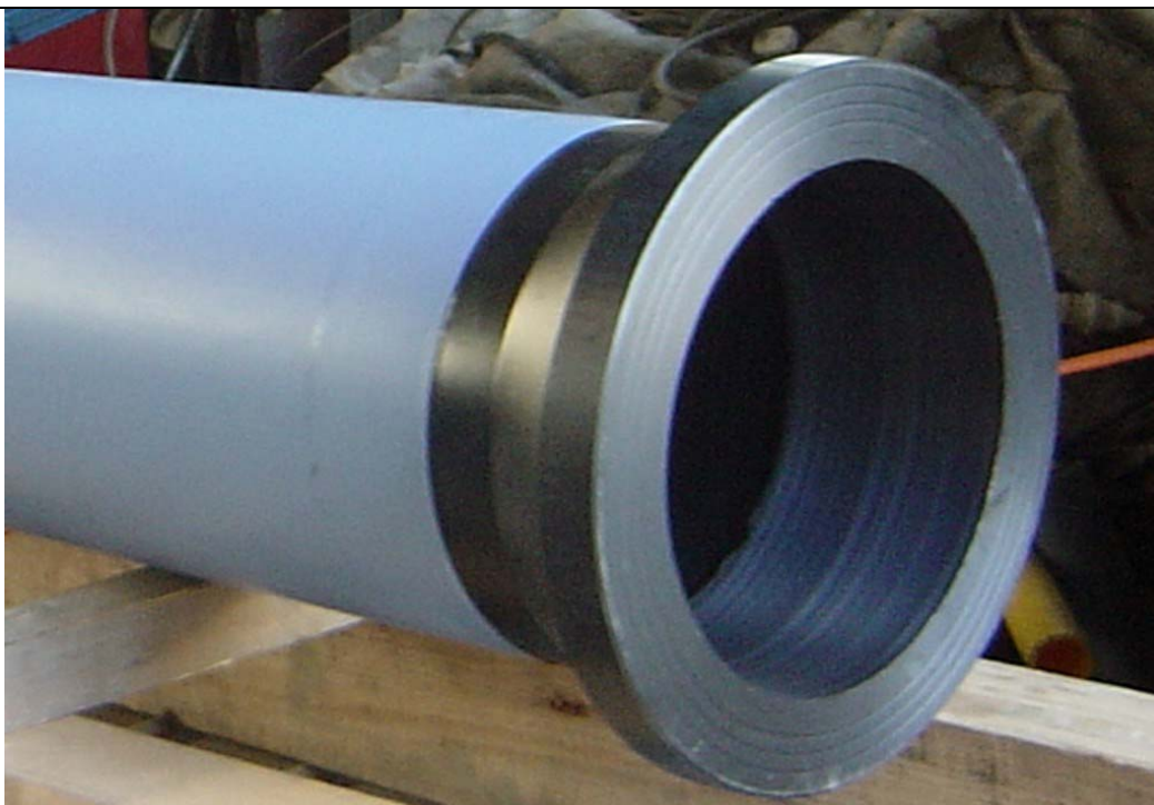
Stub End Fitting Connection
